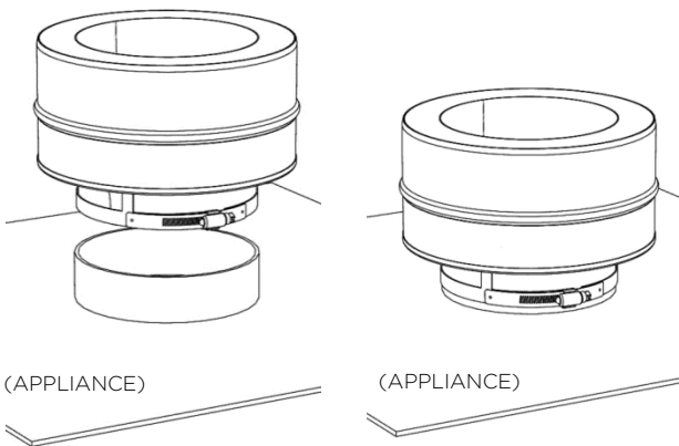
Figure 5-2, Raw Collar Adapter (Outside) Start
