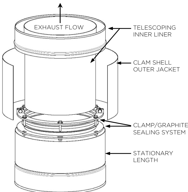
Figure 3-6, ALG Adjustable Length Model DWKL Assembly
