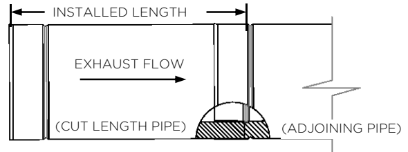
Figure 3-5, Cut Pipe Length Joint Detail
