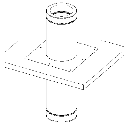
Figure 6-10, Firestop
