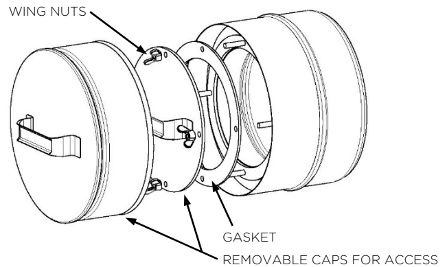
Figure 4-10, Tee Cap Access
