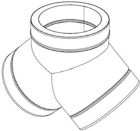
Figure 4-8, 90° Wye Tee
