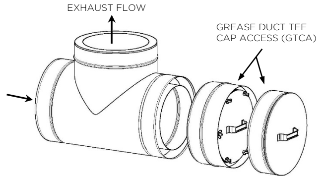
Figure 4-5, 45°, 87°, & 90° Grease Duct Tee
