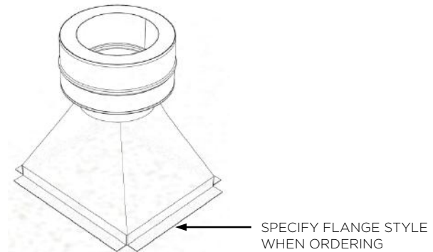
Figure 5-4, Transition to Round Start & End
