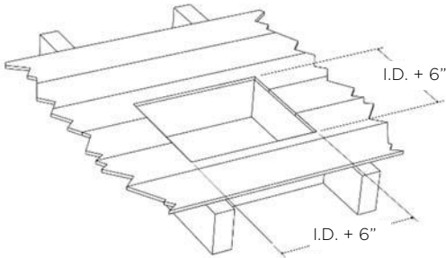
Figure 6-2, Roof Framing for Insulated Thimble
