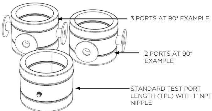
Figure 3-2, Test/Nozzle Port Section
