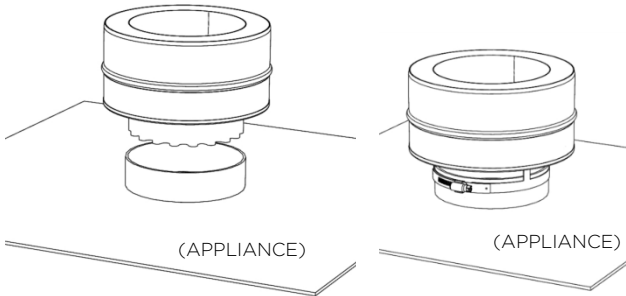
Figure 5-1, Raw Collar Adapter (Inside) Start & End
