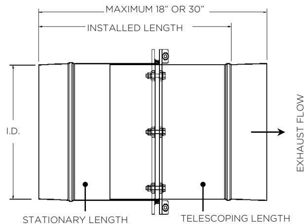
Figure 3-8, 18" & 30" ALG Adjustable Length Dimensions
