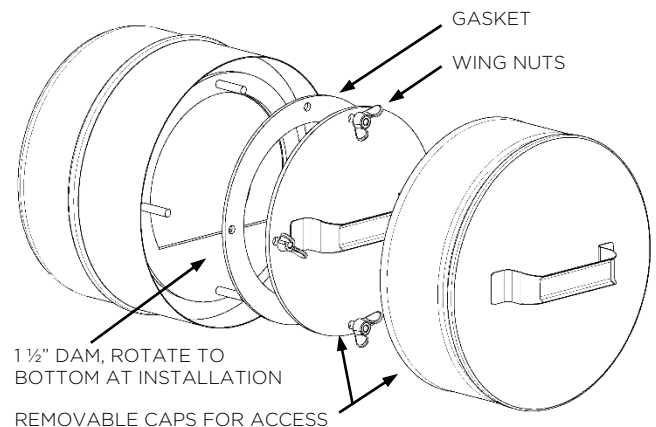
Figure 4-11, Tee Cap Access
