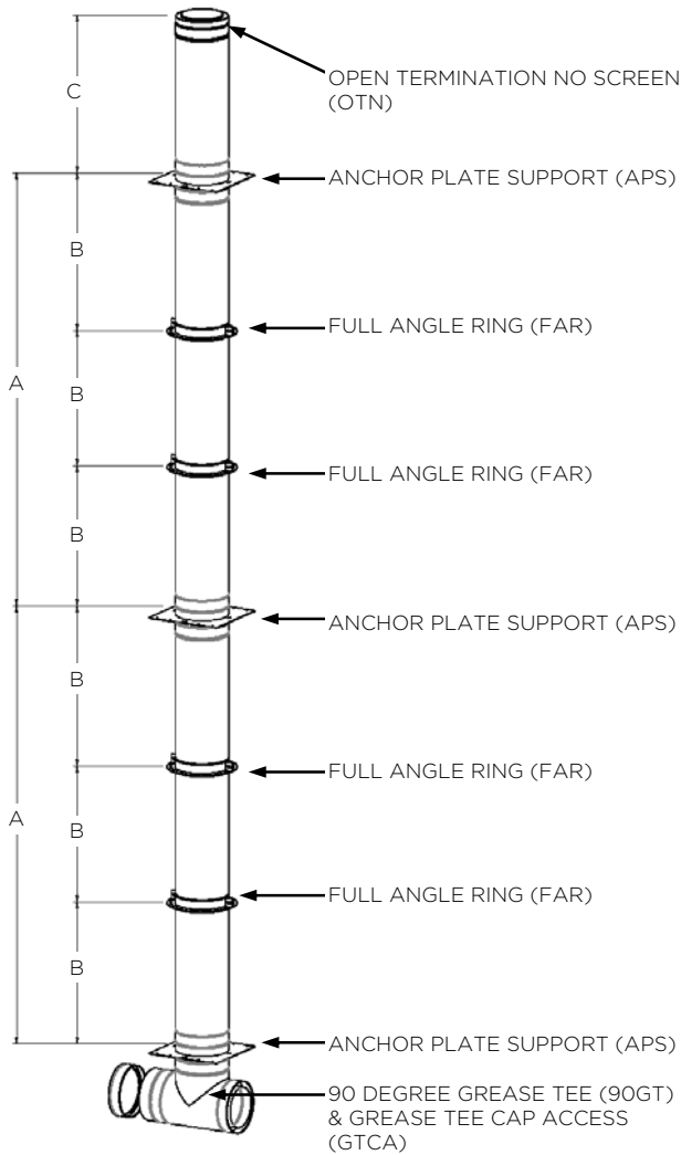
Figure 2-1, Maximum Vertical Support Spacing
