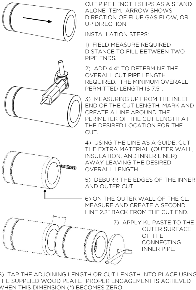
Figure 3-4, Cut Pipe Length Installation
