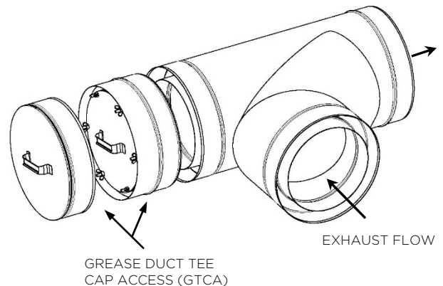
Figure 4-6, 45°, 87°, & 90° Grease Duct Boot Tee
