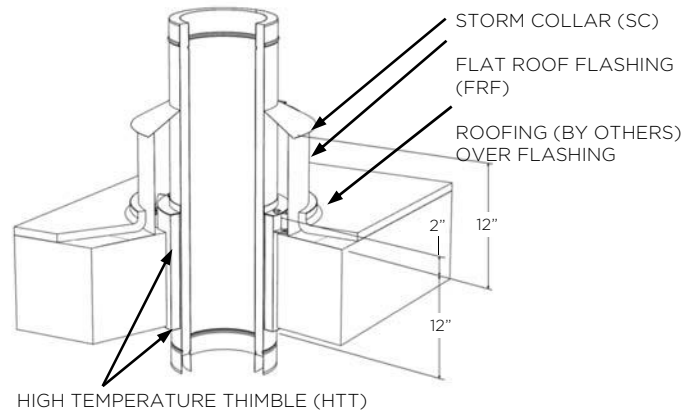
Figure 6-4, Unvented Roof Assembly
