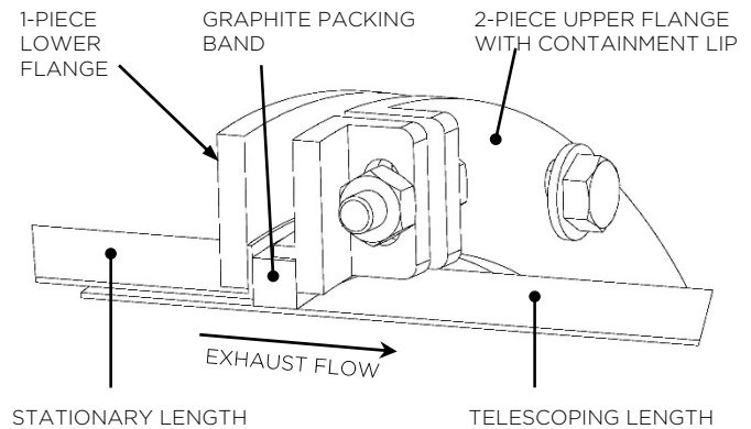
Figure 3-7, Adjustable Length Clamp/Graphite Sealing System Detail
