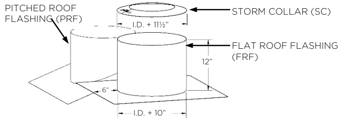
Figure 6-3, Flat & Pitched Roof Flashing and Storm Collar
