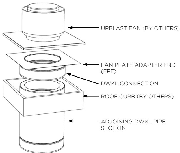
Figure 5-5, Fan Plate Adapter End
