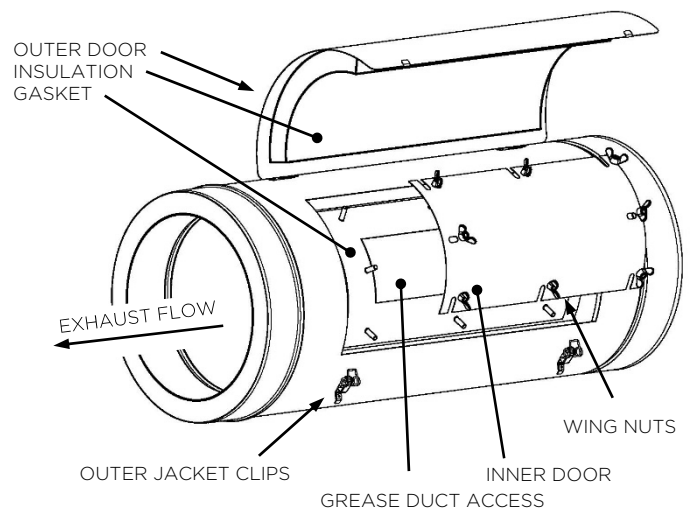
Figure 3-3, Inline Access Door
