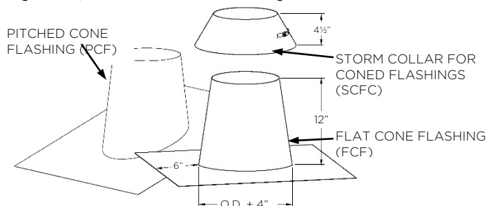
Figure 6-5, Flat & Pitched Cone Flashings and Storm Collar
